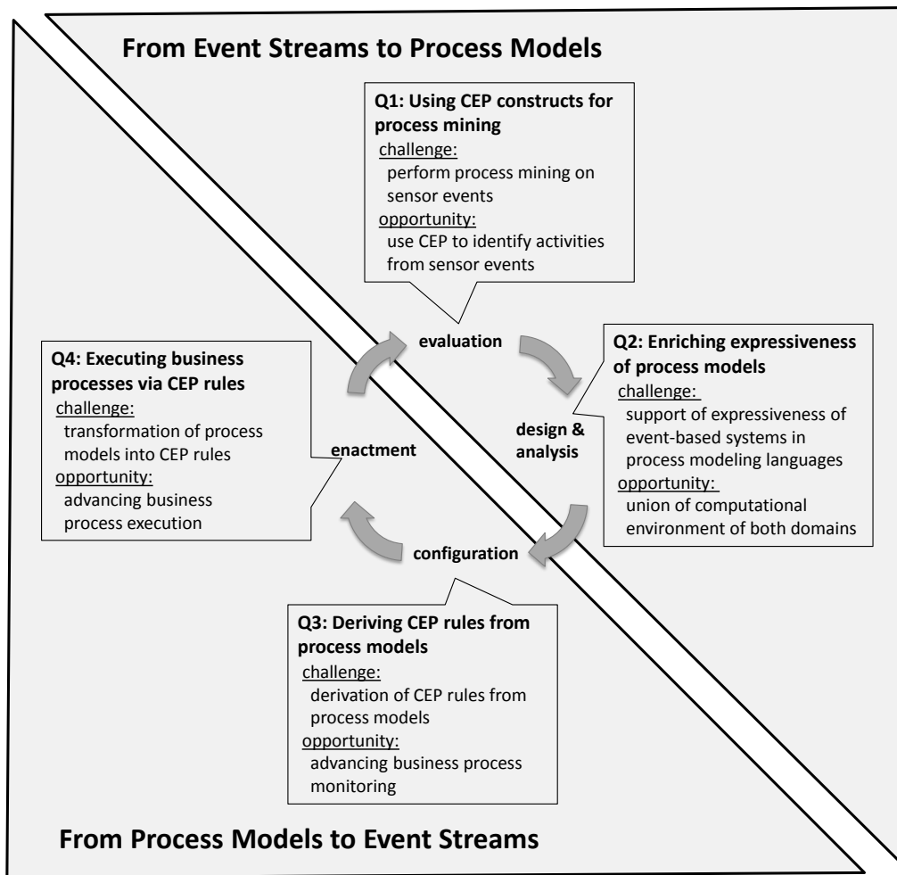
Figure 5: Four key quadrants of combining BPM and CEP concepts
