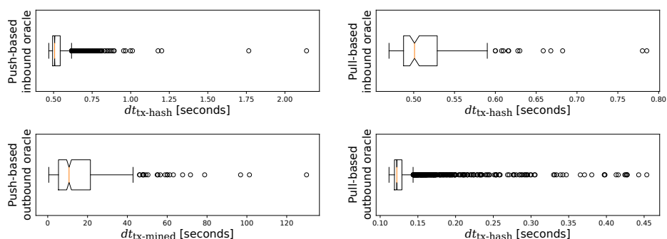
Fig. 11. Performance plots for the four oracle implementations.
